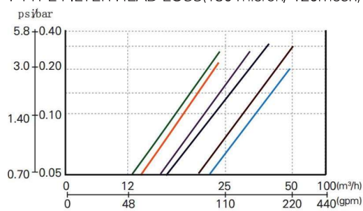
T TYPE FILTER HEAD LOSS(130 micron/ 120mesh)
